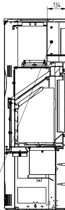
SECTION B-B
